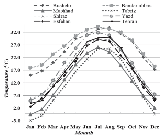
Fig. 6 Average monthly temperature of Bushehr, Bandar abbas, Mashhad, Tabriz, Shiraz, Yazd, Esfahan and Tehran during the year
