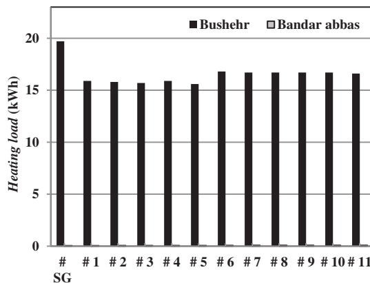
Fig. 10 Total annual heating load of office building, Bushehr and Bandar Abbas
