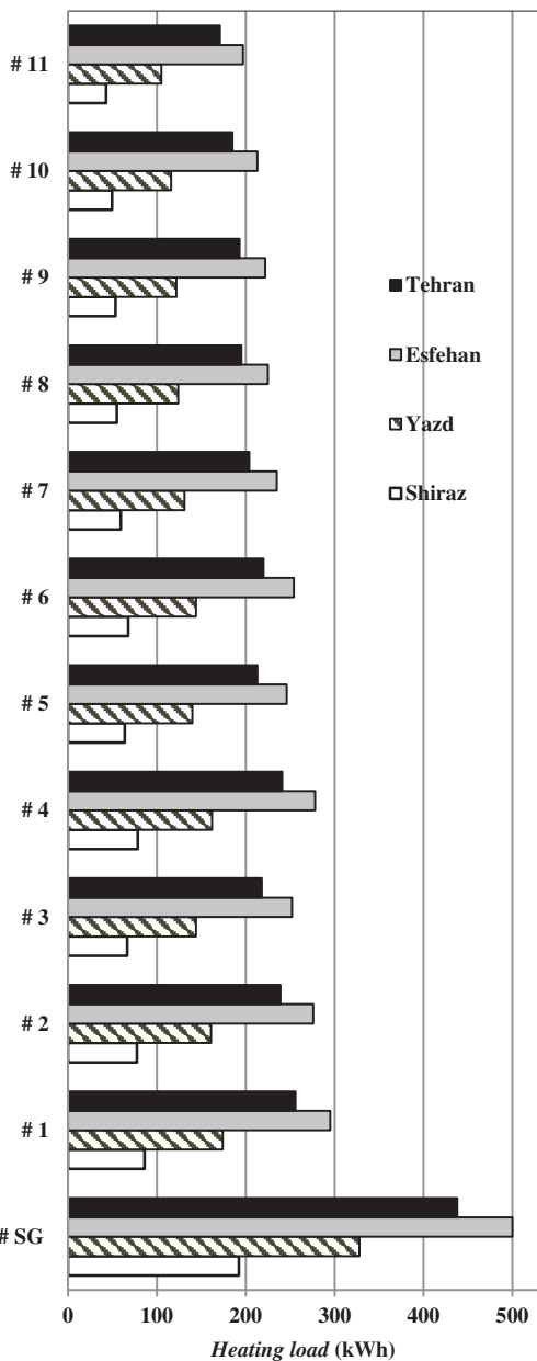
Fig. 12 Total annual heating load of office building, Tehran, Esfahan, Yazd and Shiraz
