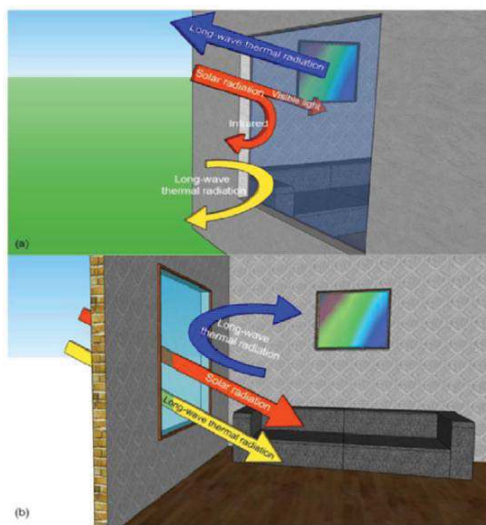
Fig. 4 Properties of ideal window for hot climates (a) and cold climate (b) (Source: Long & Ye, 2014: 2)
