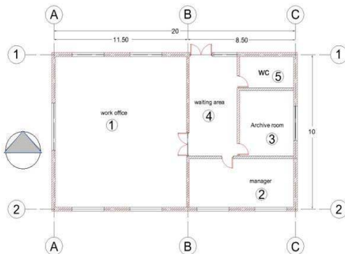
Fig. 7 Plan of office building for simulation
