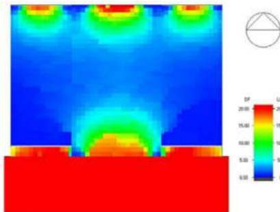
Fig. 11 Trombe wall with Conservatory
