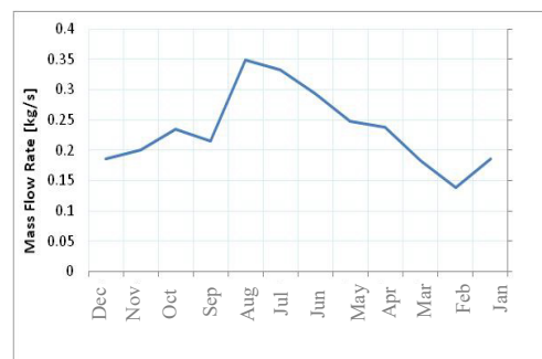
Fig.20. Total flow of solar chimney model two in one year
