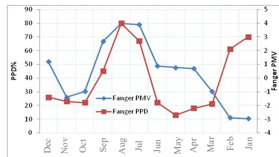
Fig.9. One year PMV and PPD values from thermal performance of solar chimney from model one for room space on the fourth floor
