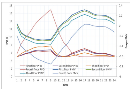
Fig.10. Comparison of PMV and PPD characteristics for four model floors on 1. May
