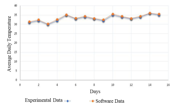
Fig.3. Daily average temperature correlation test (11:15 - 11:30)
