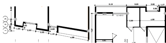
Fig. 11. Deep window on the north and south facades of the building
