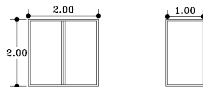
Fig. 21. Dimensions 2 \times 2 and 1 \times 2 on the north side of the building and windows with dimensions 2 \times 2 on the south side
