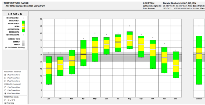
Fig. 2. Bushehr air temperature in comparison with thermal comfort conditions
