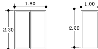
Fig. 22. Dimensions 2.20 \times 1.80 and 1 \times 2.20 on the north side of the building and a window measuring 1.80 \times 2.20 on the south side
