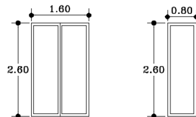
Fig. 23. Dimensions 2.60 \times 1.60 and 0.8 \times 2.60 on the north side of the building and a window measuring 1.60 \times 2.60 on the south side of the building
