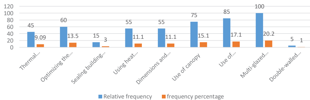
Fig. 11. Frequently distribution of energy consumption reduction solutions in envelope design
