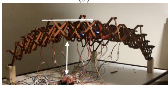
Fig. 12. Adaptation stages of the laboratory model under the stimulation of light radiation to the optical sensor simulating sunlight
